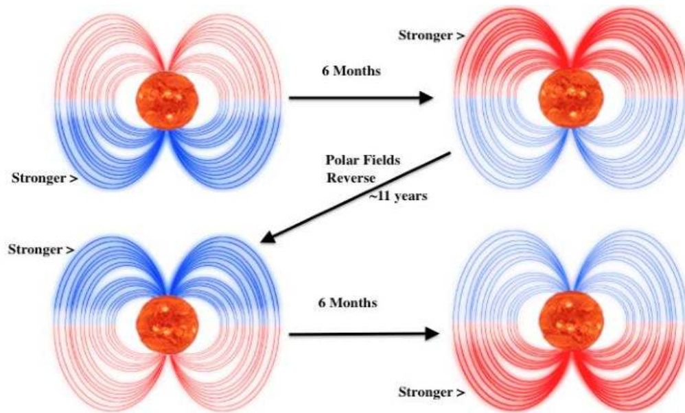
Fig. 2. Visual Representation of the ~1-year/~11-year Oscillations of the SPF. The top two images represent the shifting between N and S polar field strength, usually ~6 months apart. Top left we see thicker, bolder blue lines, representing stronger force to the southern pole. Top right we see thicker, bolder red lines, representing stronger force to the northern pole. The bottom two images are after a pole reversal has taken place, which occurs every ~11 years, and represent the same pattern of magnetic force alternating between N and S.
