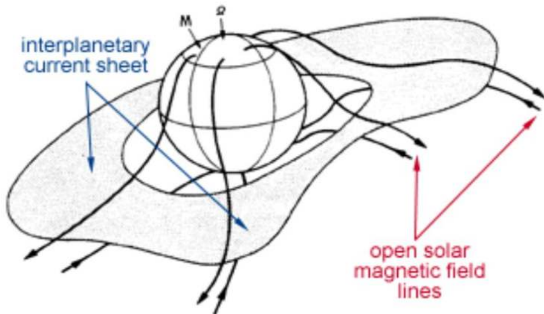
Fig. 5. Lowest-Latitude Polar Fields Interact With Solar Wind. The lowest-latitude polar fields are interacting with the current sheet, and the Earth's orbit takes it through the north/south expanse of the sheet. "The cartoon showing the tilted current sheet and open solar magnetic field lines is adapted from Smith et al., Observations of the interplanetary sector structure up to heliographic latitudes of 16 degrees: Pioneer 11, J. Geophys. Res. , v. 83, no. 717, 1978. The artist's conception of the heliospheric current sheet was obtained from J. Todd Hoeksema, Stanford University." xuv.byu.edu/docs/previous_research/euv_imager/documentation/part3/3IMF.html .
