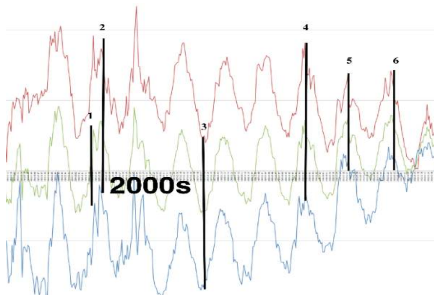
Fig. 4. The Six Largest Earthquakes of the Current Solar Polar Fields Cycle. A close-up of the Polar Maximum of the 2000s/2010s with black vertical lines at the 6 largest earthquakes of this the period. 5 of the 6 fell within 'Significant Windows'. (1) M9.1 Sumatra. December 26, 2004. Occurred during an "Average Reversal." (2) M8.6 Sumatra. March 28, 2005. Occurred during a positive peak of the southern field. (3) M8.5 Sumatra. September 12, 2007. Occurred during a negative peak of the northern field/positive trough of the southern field. (4) M8.8 Chile. February 27, 2010. Occurred during a positive peak of the southern field/negative trough of the northern field. (5) M9.0 Japan.
