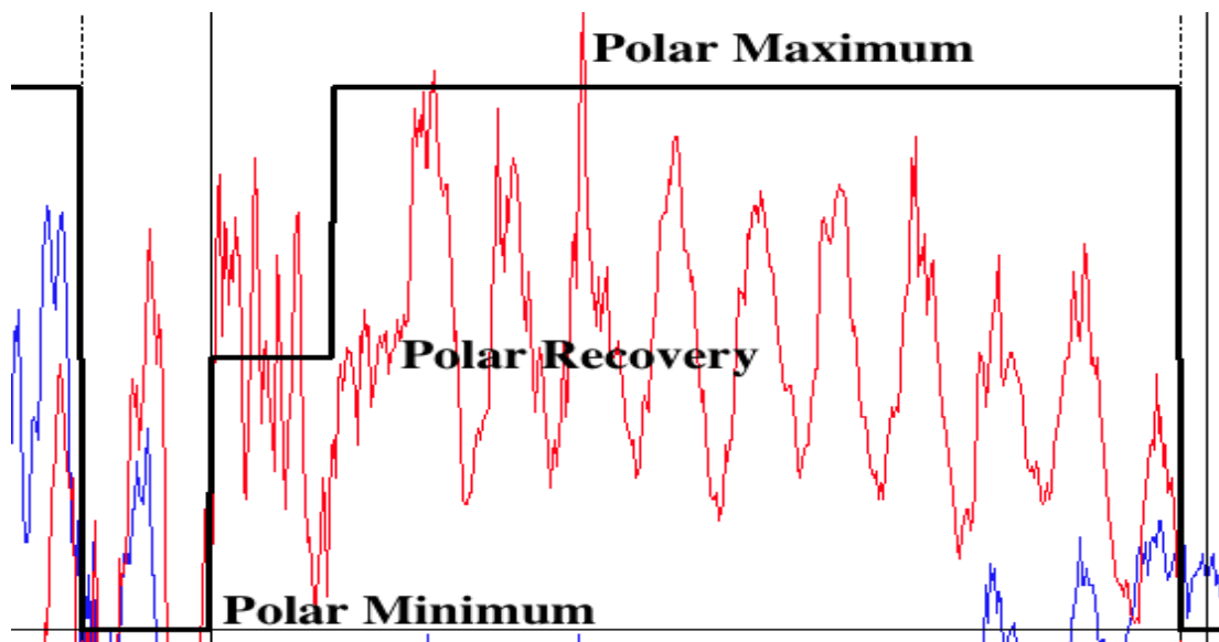
Fig. 3. Example of the Separation of Phases in the Solar Polar Fields Cycle. Polar Minimum, Recovery, and Maximum are shown here using a portion of the SPF data. The minimum shown here is the reversal that occurred from 1999-2001, followed by ~18 months of recovery, and then the maximum period. The full SPF data, broken down into the SPF phases can be seen in Appendix B. This pattern holds true for both poles, during both positive and negative phases of their cycles.
