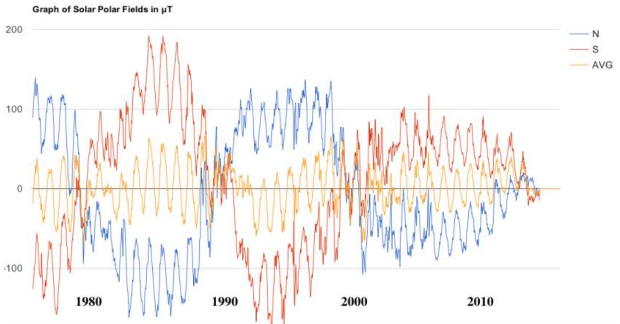
Fig. 1. Graph of Solar Polar Fields in \mu\text{T} . Solar Polarity Data adapted from the website of the Wilcox Solar Observatory. The Blue line is the North SPF, while the Red line is the South SPF. The Yellow line represents the Average Polar Magnetism of the two fields. Here we see a sinusoid on a large scale ( \sim 11 year solar cycles) and a small scale ( \sim 1 year). The Y-axis and baseline around which the solar poles are plotted is 0 \mu\text{T} . Above the baseline is positive polar magnetism, and below the baseline is negative polar magnetism - the further the line goes up or down, away from the central baseline, the stronger the magnetism.
