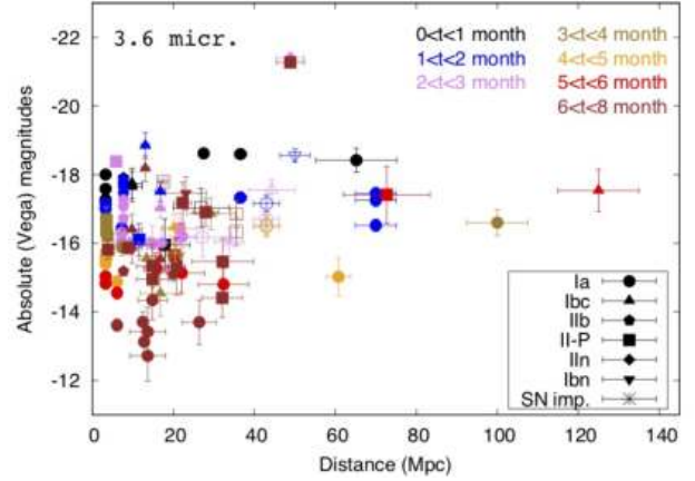
Figure 2. Early-time MIR evolution of all historical SNe obtained from Spitzer archival data by Szalai et al. (2019). Filled and open symbols denote SNe where photometry was obtained with or without image subtraction, respectively. SN subtypes (e.g., Filippenko 1997) are denoted in the legend, and “SN imp” refers to SN impostors.
