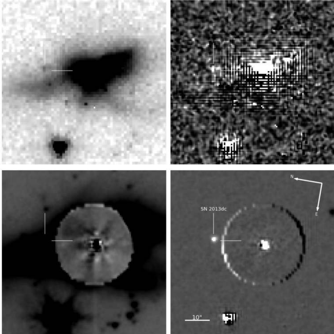
Figure 3. Comparison of sample data products, in this case for the first epoch of NGC 6240, used in our transient search. ( Top left: ) Original, unprocessed MOPEX processed data. ( Top right: ) Standard alignment and subtraction of two epochs. ( Bottom left: ) Forward modeling subtraction, where the circle corresponds to our forward modeling radius. ( Bottom right: ) Subtraction of two epochs that have been forward modeled, but in this case are spaced nearly one year apart so that the telescope roll angle is similar. The colour scale and stretch is constant for all subtracted images shown in this figure. The point source is SN 2013dc. It is present in all the images, but is most clearly detected in the bottom right. The central source is the galaxy nucleus. As described in the text, there are a number of caveats for modeling the inner core, including nonlinearity concerns. Correcting those issues is beyond the scope of this paper, but we account for them in our statistics.
